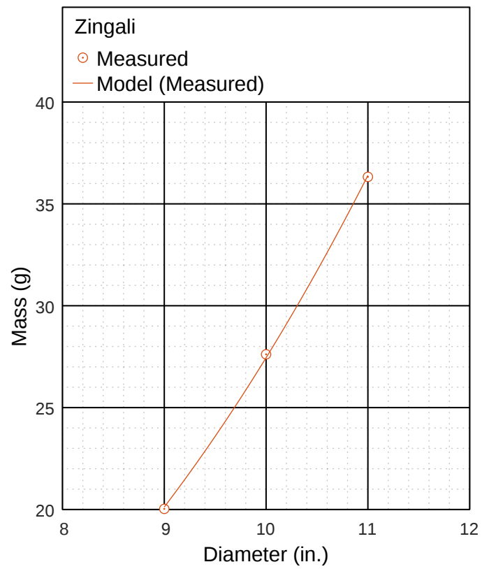
Figure 66: Zingali model.
